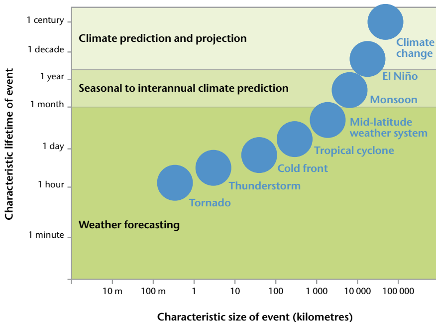
Figure 1.1. Time and space scales of weather and climate
