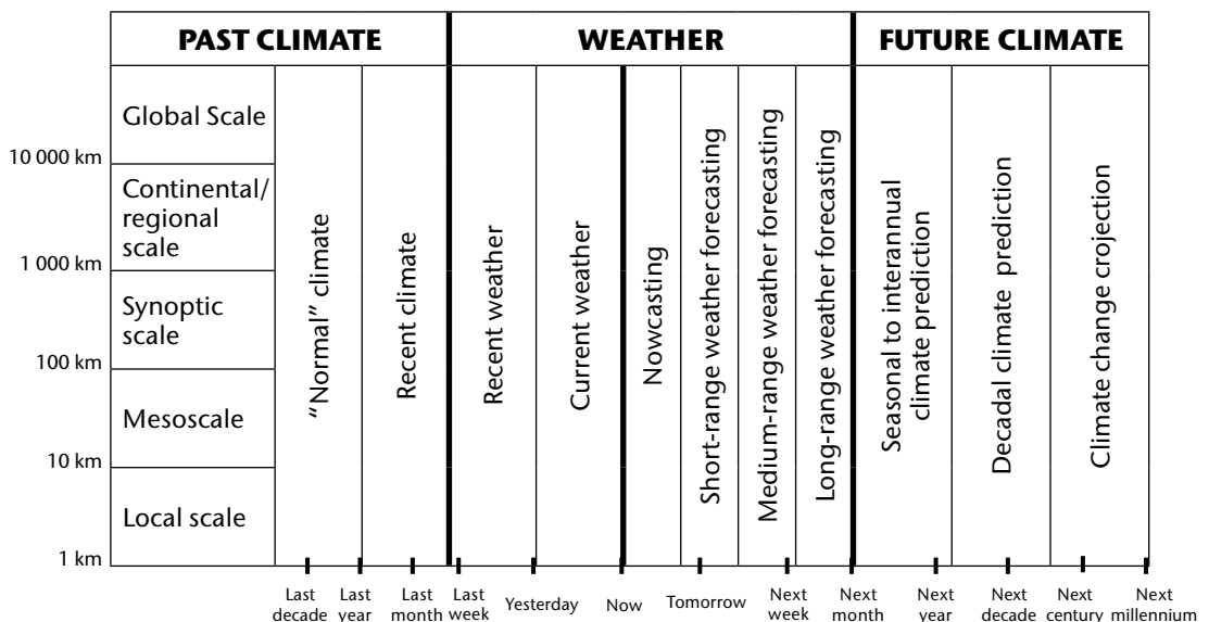
Figure 2.2. Characteristic spatial scales of weather phenomena (left-hand scale) and the approximate temporal terminology for weather and climate description and prediction (bottom scale)
