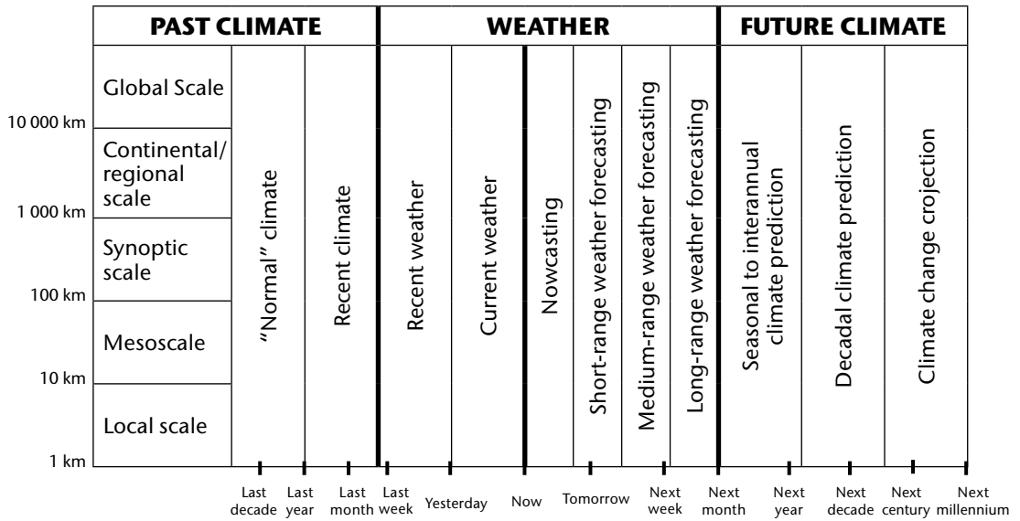
Figure B.3. Characteristic space scales of weather phenomena (left-hand scale) and the approximate timescale terminology for weather and climate description and prediction (lower scale)
